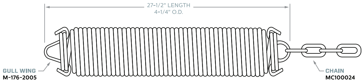
THRALL RACK DECK SPRING ASSEMBLY (typical) F0930001 WITH CHAIN F0930002 20' 2" DECK SPRING ASSEMBLY MC100040 CHAIN ONLY
