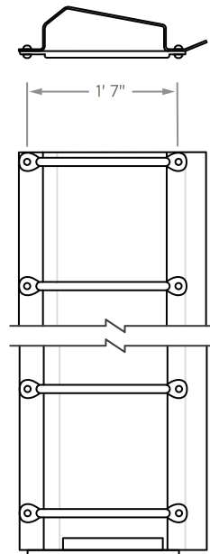
BI-LEVEL/TRI-LEVEL (UPSILL) 12' 4-3/8" LENGTH, 9 RUNGS A0020065 BL/AR A0020066 BR/AL
