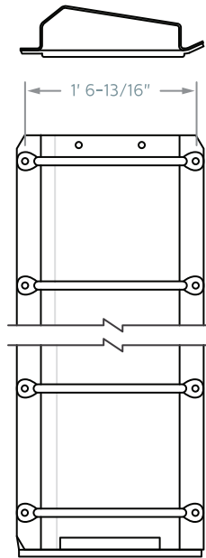
TRI-LEVEL (UPSILL) 12' 2-5/8" LENGTH, 9 RUNGS A0020014 BL/AR A0020015 BR/AL
