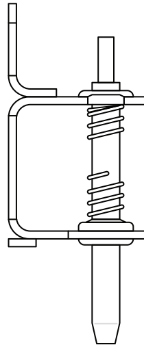
UPPER LOCK PIN ASSEMBLY BR/AL (shown) D-076-2006 BR/AL D-076-2007 BL/AR
