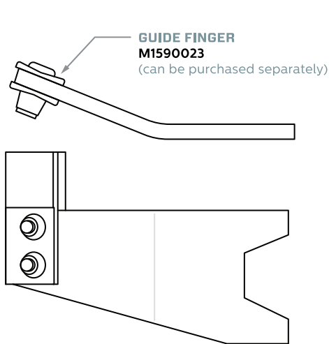
UPPER DOOR GUIDE D0130021 BL/AR D1180008 (Bracket only) TRI-LEVEL & BI-LEVEL
