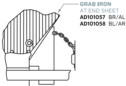
CHAIN ATTACHMENT ON CORRUGATED GALVANIZED CANOPY
