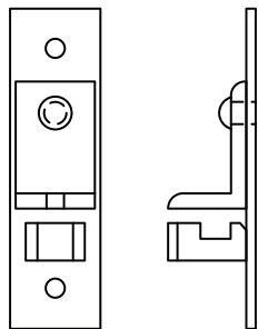
HASP LOCK ON BL/AR DOOR D-099-2025
