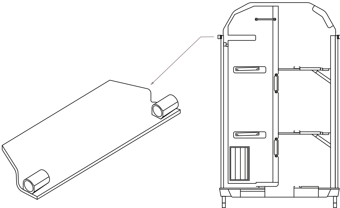
BRIDGE PLATE SUPPORT MM100681
