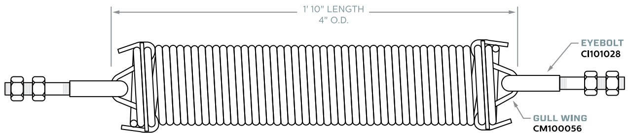
PARAGON RACK DECK SPRING ASSEMBLY (typical) (with eyebolts & hex nuts) MB100086
