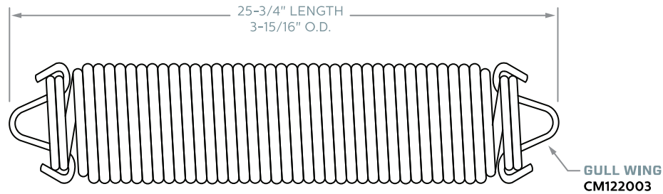
W&K RACK DECK SPRING ASSEMBLY (typical) MB100007
