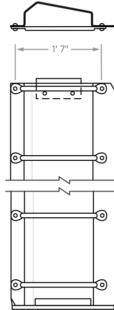
BI-LEVEL 12' 8" LENGTH, 9 RUNGS A0020036 BL/AR A0020037 BR/AL
