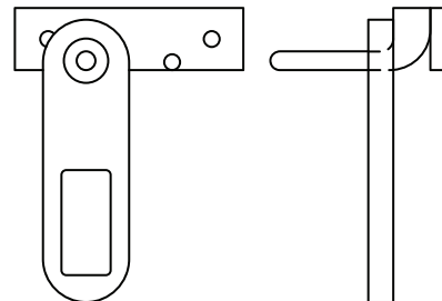
HASP LOCK ON BR/AL DOOR D-099-2024
