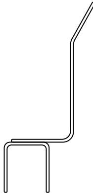
RETAINER SIDE PANEL TO ROOF RAIL (1 pc design) M1050381
