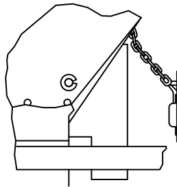
CHAIN ATTACHMENT ON HEAVY PLATE CANOPY
