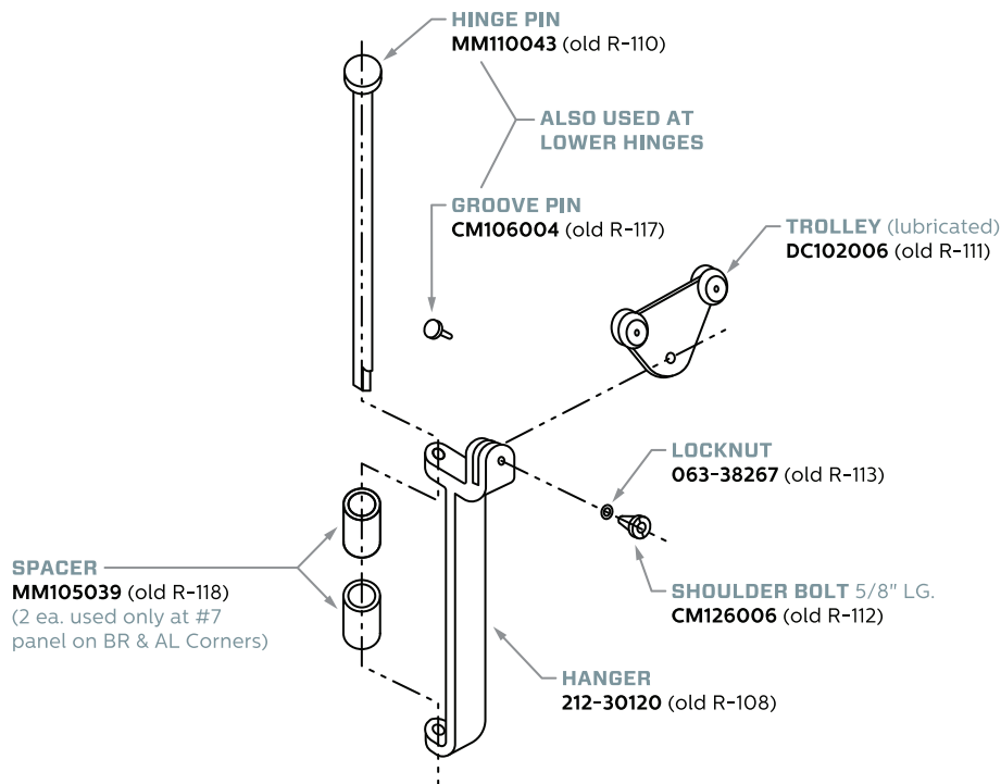
TROLLEY ARRANGEMENT #2 THRU #7 PANELS
