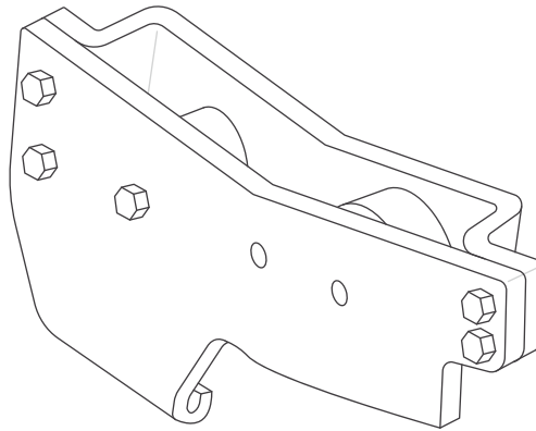
ROLLER ASSEMBLY - INNER (ORIGINAL STYLE) BL/AR (shown) D0120002 BL/AR D0120003 BR/AL
