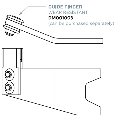
UPPER DOOR GUIDE WEAR-RESISTANT ASSEMBLY D0130025 BL/AR (reduced slot & slotless door) D1180018 (Bracket only)
