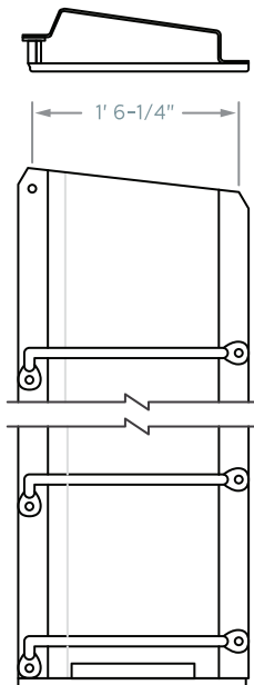
TRI-LEVEL 12' 5-3/8" LENGTH, 8 RUNGS A0020012 BL/AR A0020013 BR/AL
