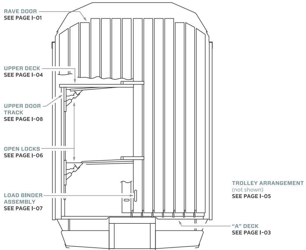
END VIEW (TRI-LEVEL)
