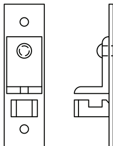
HASP LOCK ON BL/AR DOOR M0300031
