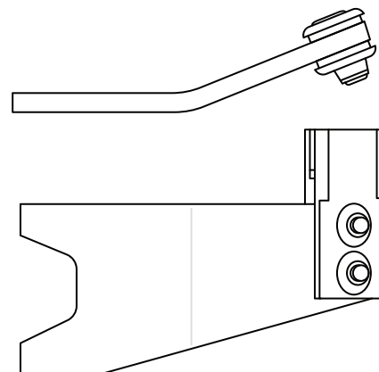
UPPER DOOR GUIDE WEAR-RESISTANT ASSEMBLY D0130026 BR/AL (reduced slot & slotless door) D1180019 (Bracket only)
