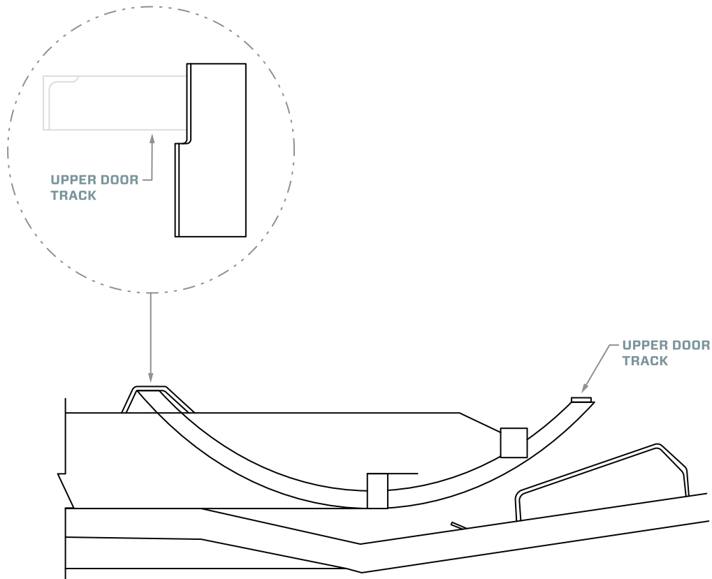
SAFETY SHIELD (closure at Shear Panel opening for Upper Door Track) A1210016 BL/AR A1210017 BR/AL
