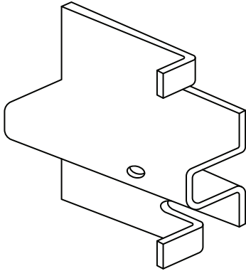
RETAINER ATTACHED TO SIDE POST 9/16" HOLE M-226-2180
