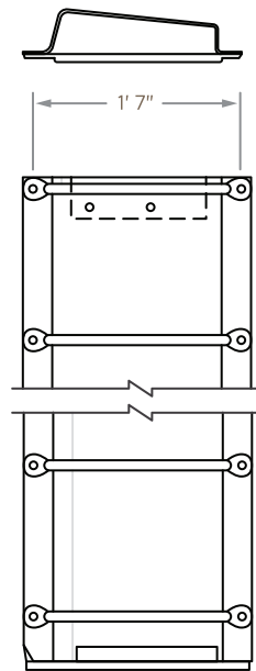
BI-LEVEL 12' 6-1/2" LENGTH, 9 RUNGS A0020006 BL/AR A0020007 BR/AL
