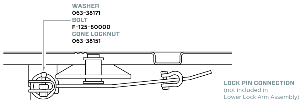
LOWER LOCK ARM INSTALLED TOP VIEW
