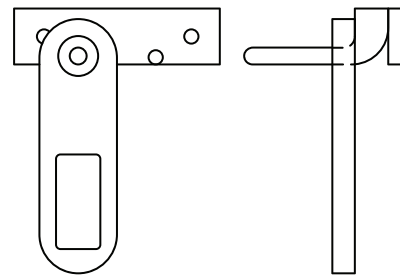
HASP LOCK ON BR/AL DOOR D-099-2024
