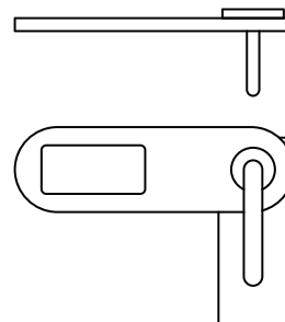
HASP LOCK ON BR/AL DOOR M0300024
