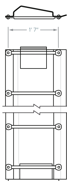
TRI-LEVEL 14' 7-3/8" LENGTH, 11 RUNGS A0020076 BL/AR A0020077 BR/AL
