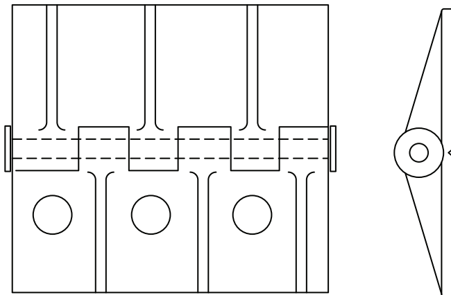
HINGE (Thrall) M0280007 HINGE PIN ROD M1630006
