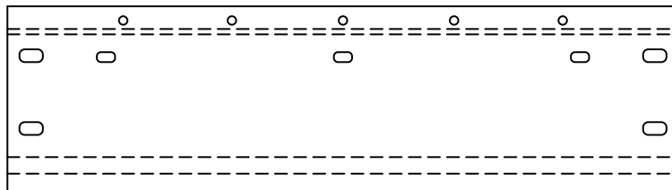
COVER SKIRT (Kick Plate) SA100059 63-1/2" length SA100058 101" length
