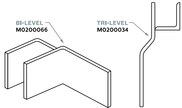
RETAINER SIDE PANEL (welded to flatcar)
