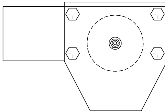
ROLLER ASSEMBLY - OUTER D0120033WA BL/AR D0120034WA BR/AL
