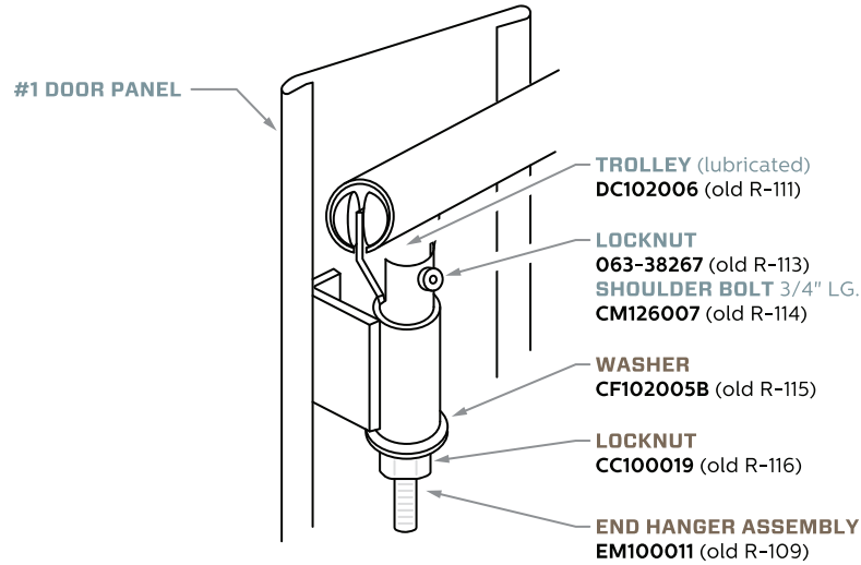
TROLLEY ARRANGEMENT #1 PANEL
