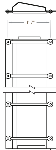
BI-LEVEL/TRI-LEVEL 12' 4-3/8" LENGTH, 9 RUNGS A0020053 BL/AR A0020054 BR/AL
