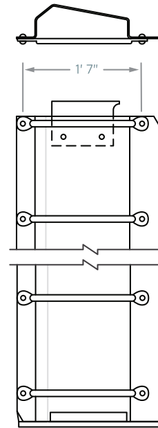
TRI-LEVEL (FLUSH DECK) 12' 9-3/8" LENGTH, 9 RUNGS A0020051 BL/AR A0020052 BR/AL
